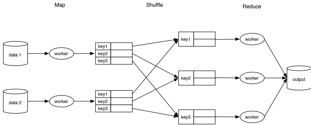
Figure 2. MapReduce model.
